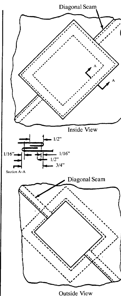
(B) Rectangular Patch Crossing A Diagonal Seam
