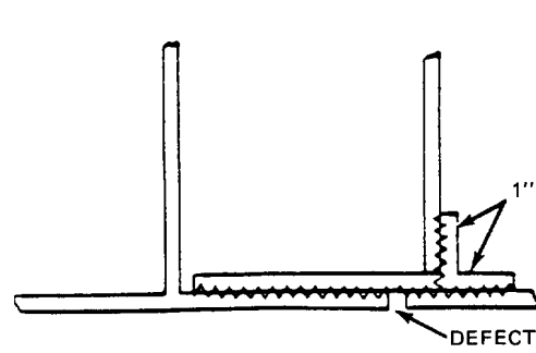
B. Repair To Bottom Cord When Defect Is Within 1-Inch Of Vertical Cord
